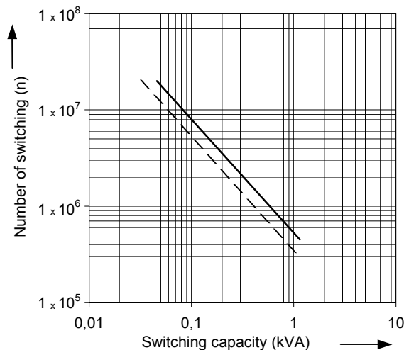
2 RH 02, 2 RH 62, 4 RH12 contact material: AgCu
